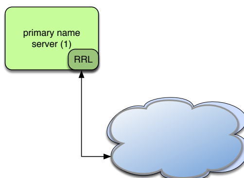
Figure 17.4: Primary name server with RRL
