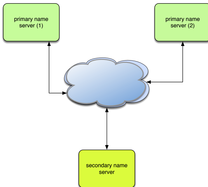
Figure 17.11: Secondary name server (several primaries)
